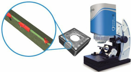
Automatic Edge Chipping Measurement with EdgeMasterX
